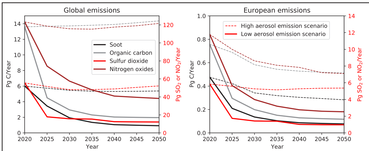
Figure 3. Future emission scenarios of soot, organic carbon, sulfur dioxide ( \text{SO}_2 , a precursor of sulfur particles) and nitrogen oxides ( \text{NO}_x , a precursor of nitrate particles). Emissions following a “low aerosol emission scenario” (Maximum Feasible Reduction) are marked with full lines while emissions following a “high aerosol emission scenario” (Current Legislation) are marked with dashed lines.
